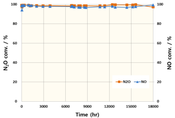
Durability of Catalyst ( at 550°C)
