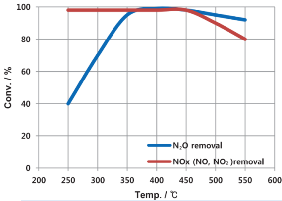
Performance of Catalyst
